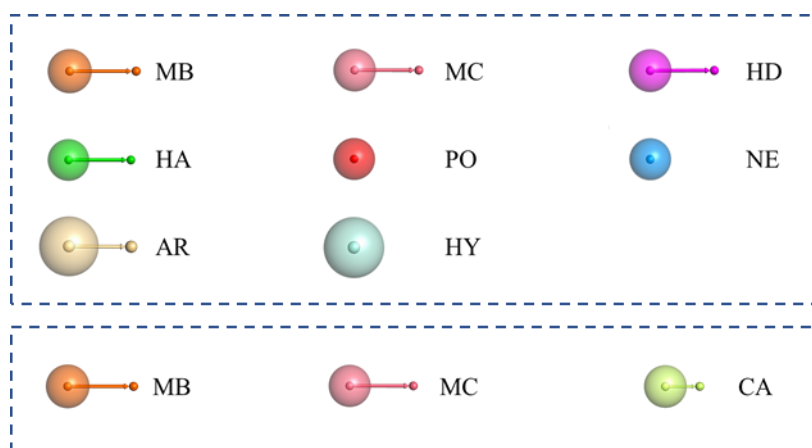
Figure 1. Graphic representation of eight types of pharmacophore features and three types of \alpha -carbon features showed by a PyMOL plugin.
