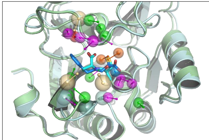
Figure 4. The superposition of 4C1E (green) and 2YZ3 (cyan) based on pharmacophore
