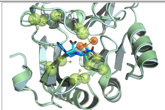
Figure 5. The superposition of 4C1E (green) and 2YZ3 (cyan) based on \alpha -carbon
